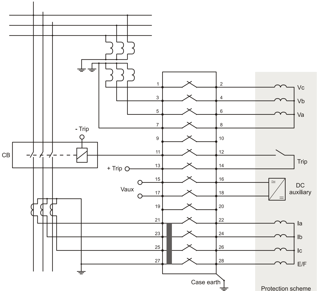
CT shunting bar for circuit isolation
