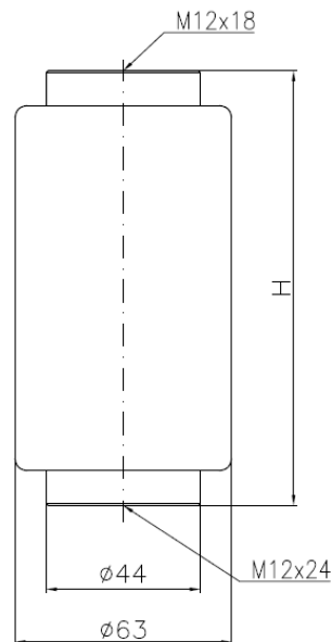
Fig. 1 Dimension drawing surge arresters type PROXAR-IIW DC
